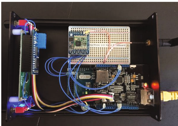
FIGURE 5: Smart alert RTU signal gateway for LoRa.
