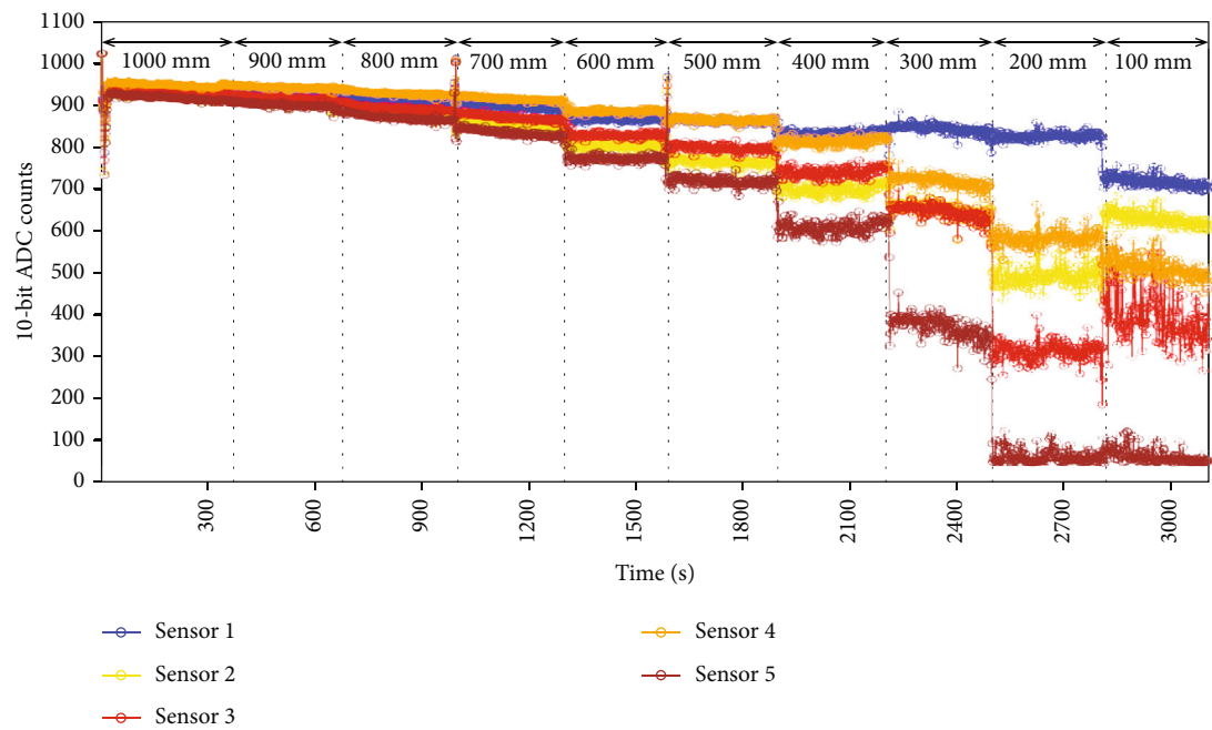
FIGURE 7: Typical fire sensor's simulation performance.
