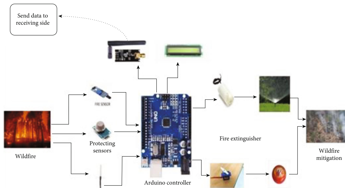
FIGURE 3: Signal/data controller of the forest unit.
