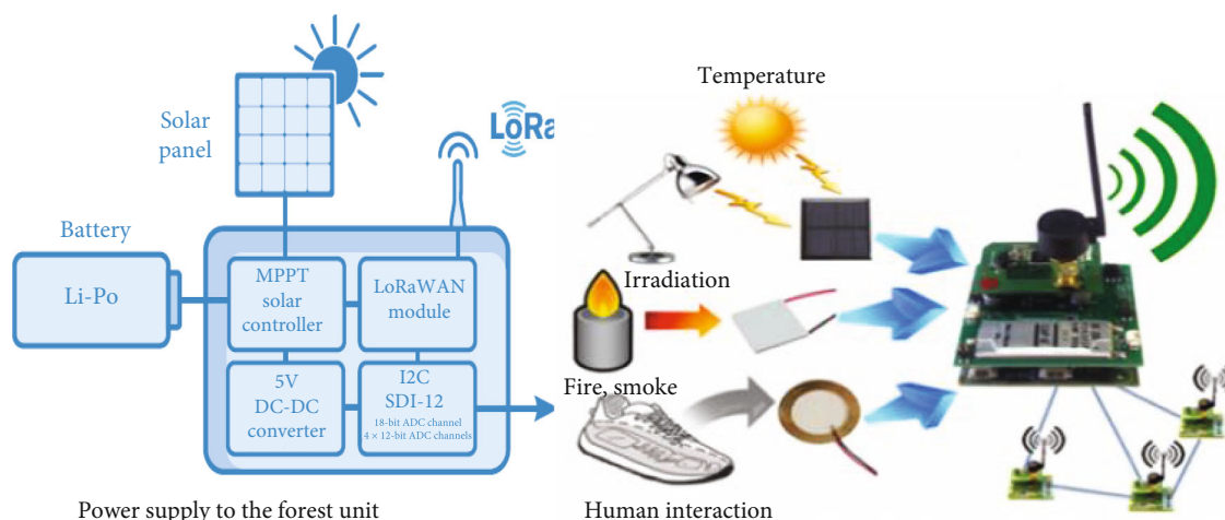
FIGURE 2: The elements of the remote access forest unit.
