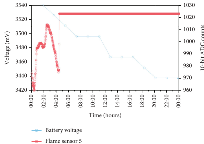
FIGURE 12: Real-time RSU's battery voltage and flame sensor data at alert monitoring screen.
