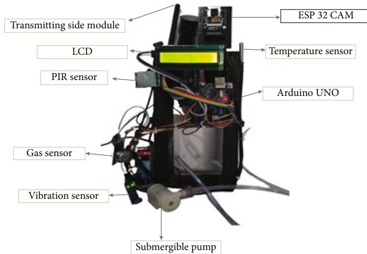
FIGURE 4: RAU (remote access unit) for the forest alert monitoring system.
