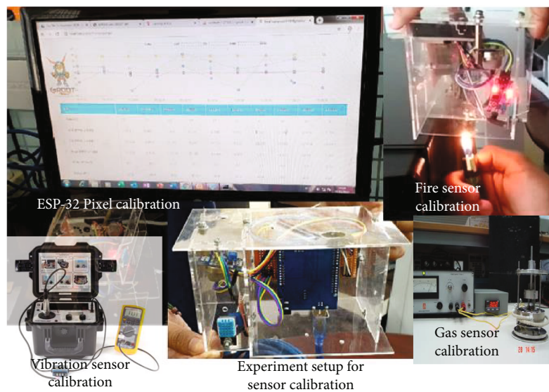
FIGURE 8: Calibrations of sensor's threshold values.
