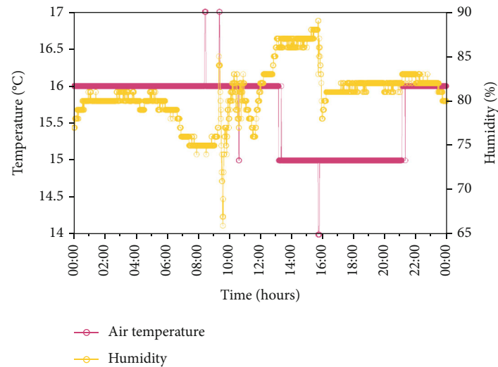
FIGURE 11: Day temperature and humidity data collected by RAU sensor at alert monitoring screen.
